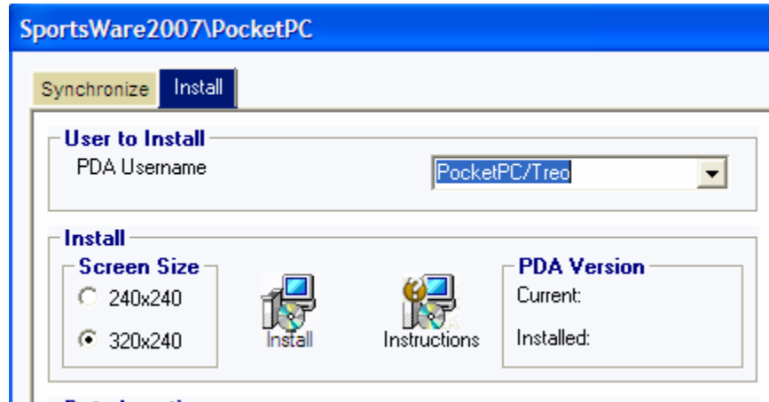
Figure 3 - Install Tab
